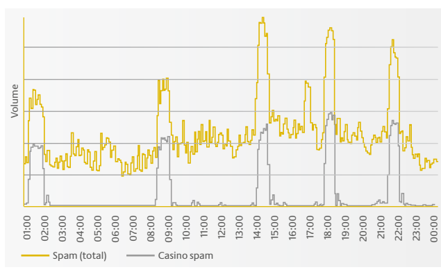
Fig. 9: Casino waves and total spam volume over a typical day [7]
