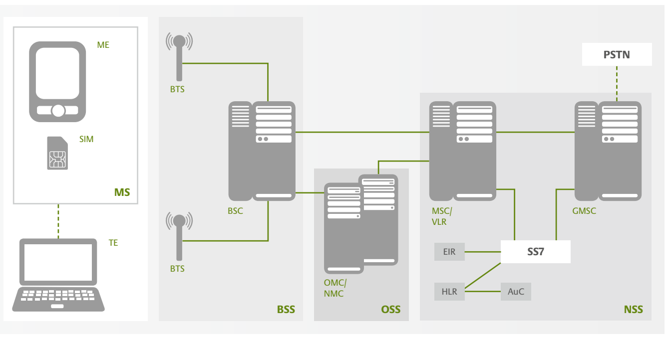
Fig. 13: Simplified diagram of a GSM mobile network [7]
