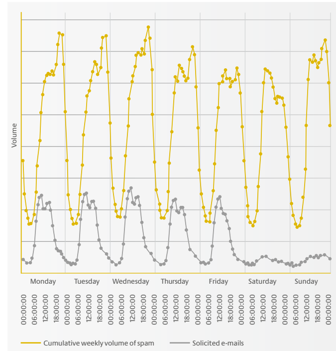
Fig. 7: Cumulative weekly volume of spam and solicited e-mails sent from Germany [7]
